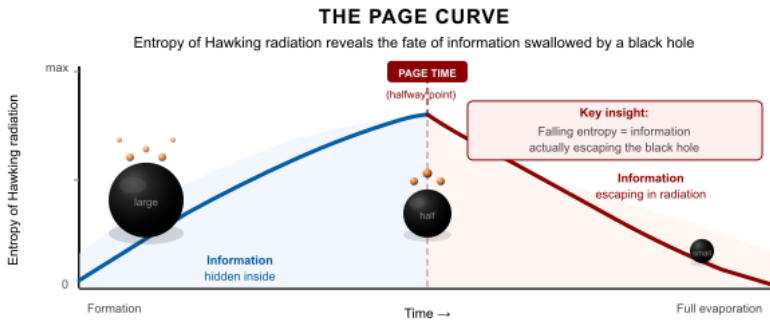
Figure 19 - 1 Key insight: Falling entropy after the Page time is the mathematical signature of information escape. If information were destroyed, entropy could only ever rise. The downward slope proves preservation.
